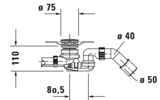
Siphon with base inlet for bathtub # 700451
