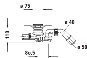
Siphon with base inlet for bathtub # 700453
