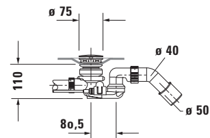
Siphon with base inlet for bathtub # 700453
