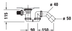
Siphon for whirltub # 760453
