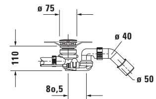
Siphon with base inlet for bathtub # 700449
