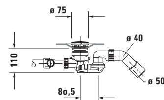
Siphon with base inlet for whirltub # 760451
