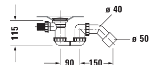
Siphon for whirltub # 760451
