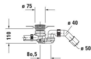
Siphon with base inlet for bathtub # 700451
