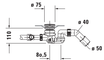
Siphon with base inlet for whirltub # 760451
