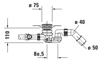
Siphon with base inlet for whirltub # 760453
