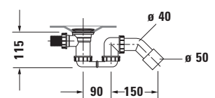
Siphon for whirltub # 760450
