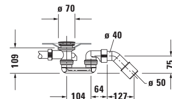
Siphon for bathtub # 700451
