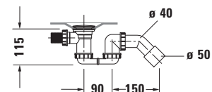
Siphon for whirltub # 760450
