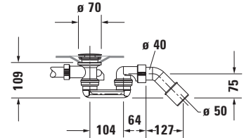
Siphon for bathtub # 700453
