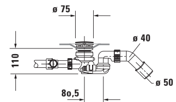
Siphon with base inlet for whirltub # 760449
