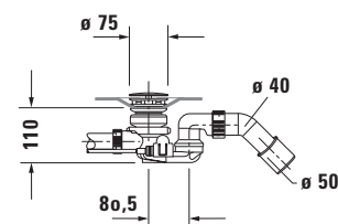
Siphon with base inlet for bathtub # 700450
