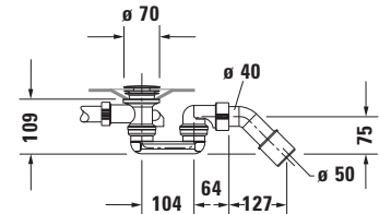
Siphon for bathtub # 700450
