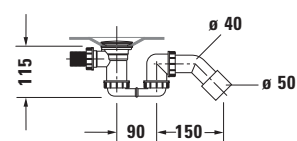
Siphon for whirltub # 760453
