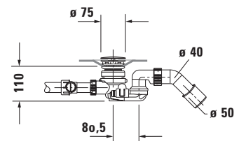
Siphon with base inlet for whirltub # 760450
