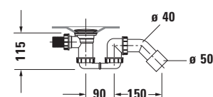
Siphon for whirltub # 760451
