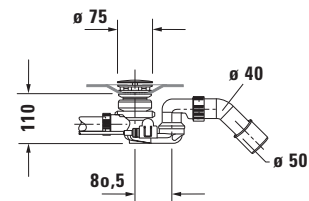
Siphon with base inlet for bathtub # 700450
