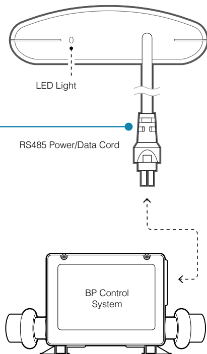
GATEWAY ULTRA Module (side view)
